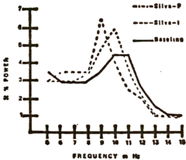
Figure II : Power spectra for Silva-trained group, showing baseline data, training data (Silva 1), and biogenic feedback data (Silva-f).
