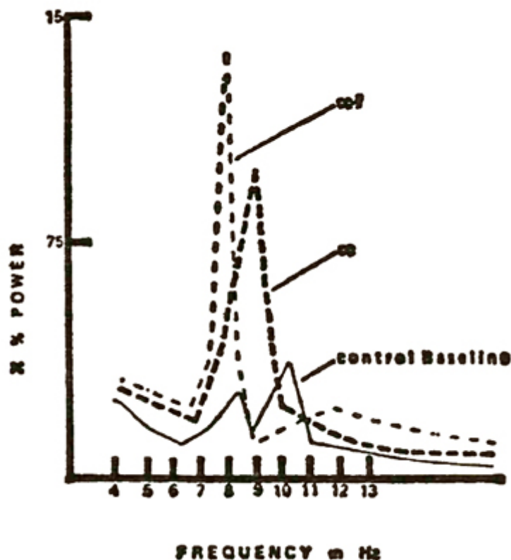
Figure I : Power spectra for the classical conditioning group, showing baseline (control), conditioning (CC), and biogenic
