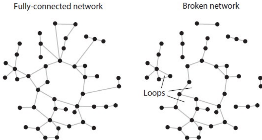
Illustration of fully-connected and broken Erdős–Rényi networks
