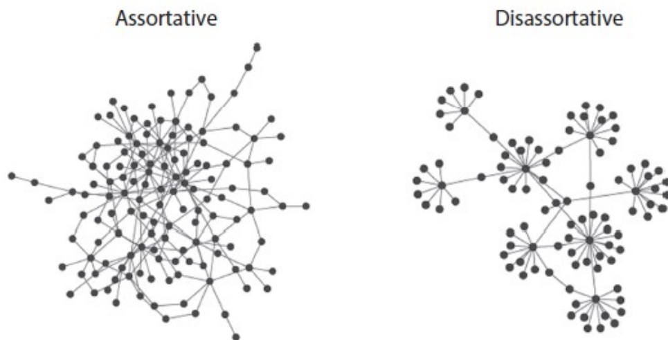
Illustration of assortative and disassortative networks
