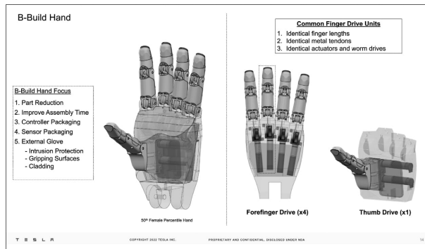
A slide showing components of Optimus's hand
